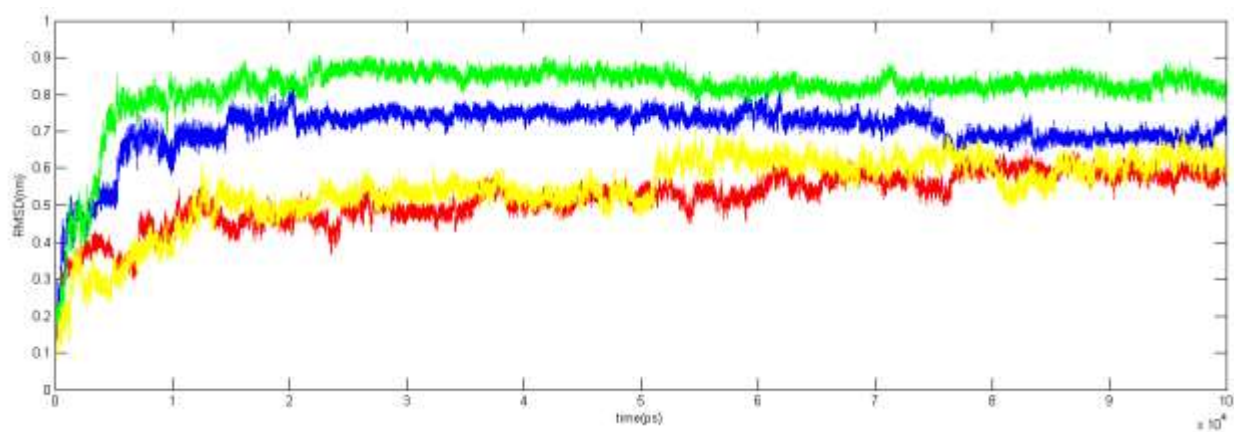
S. 1 The C\alpha -RMSD (nm) of H-NS vs. time (ps).
