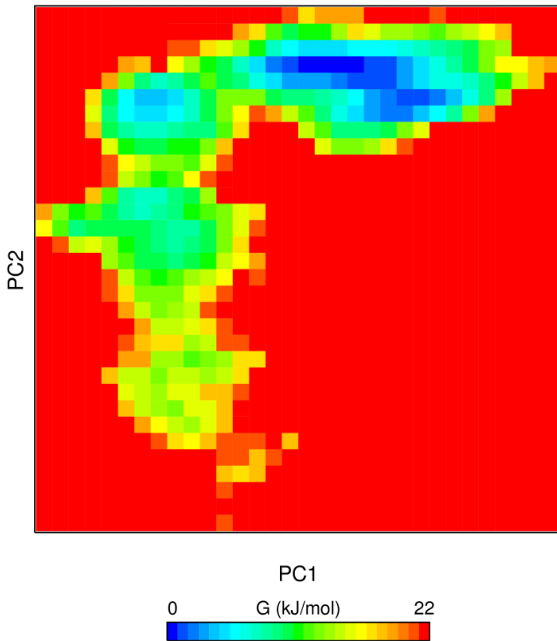
S. 4 2D Free Energy Landscape of the protein-SWCNT simulated system
