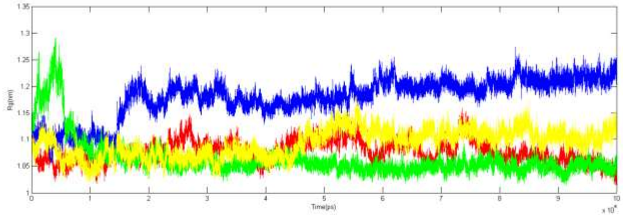
S. 2 The Rg (nm) of H-NS vs. time (ps).
