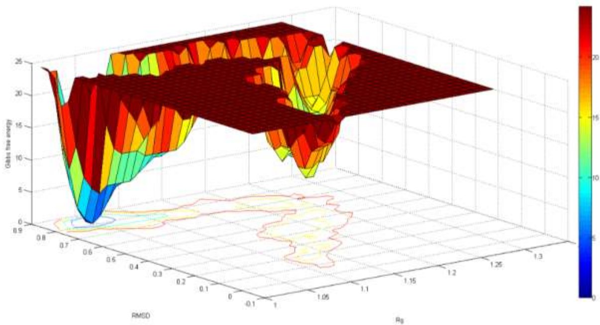
S. 9 3D Free Energy Landscape of the protein-DNA simulated system
