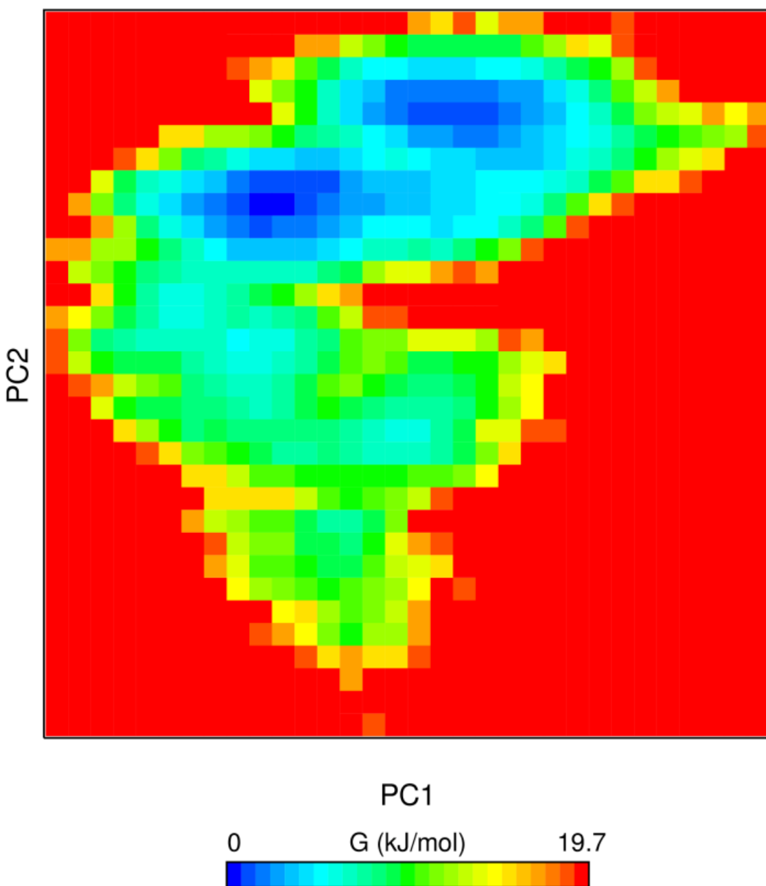
S. 6 2D Free Energy Landscape of the protein-SWCNT-DNA simulated system
