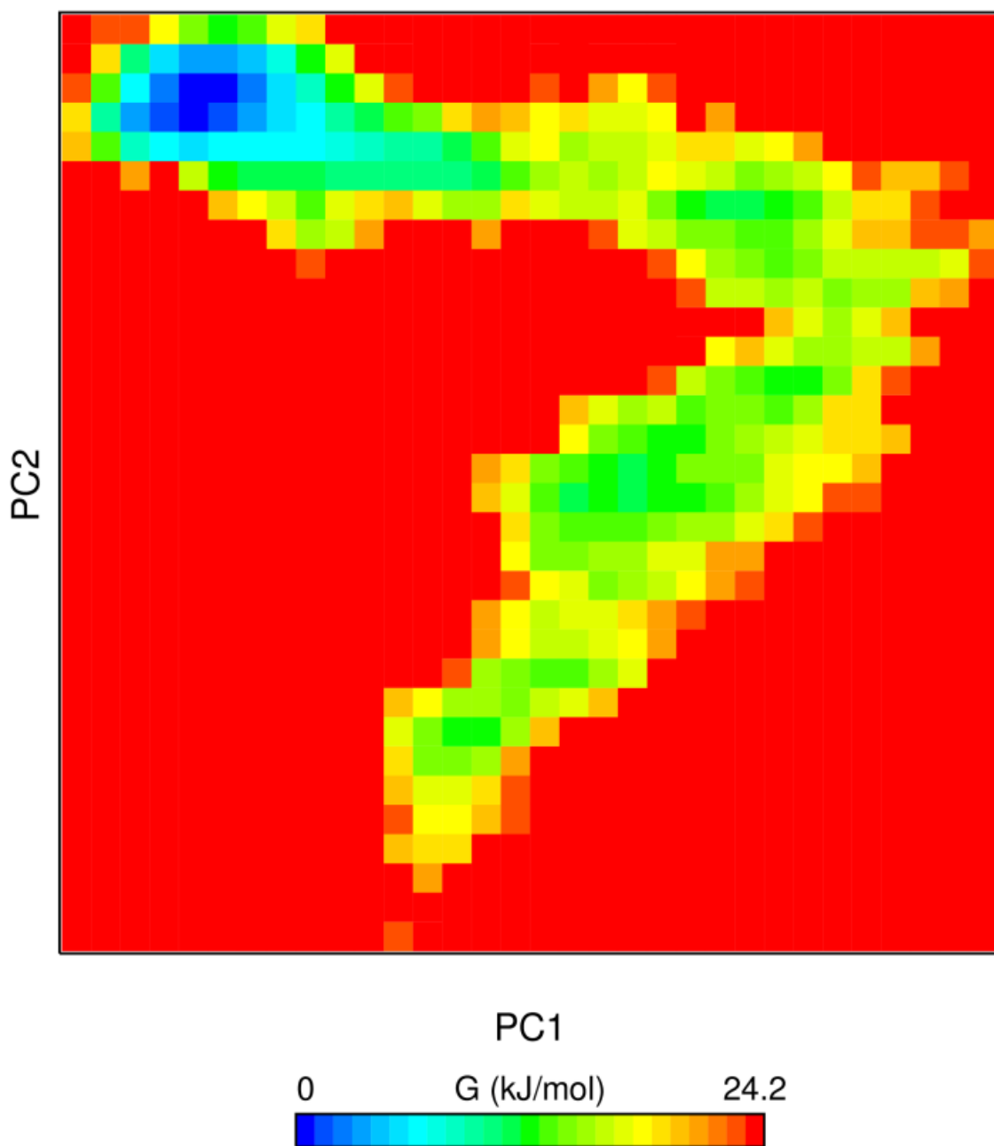
S. 5 2D Free Energy Landscape of the protein-DNA simulated system
