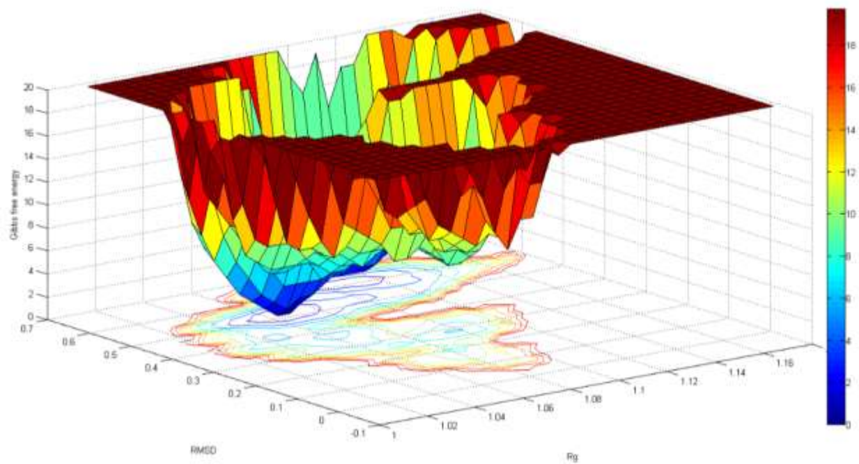
S. 10 3D Free Energy Landscape of the protein-SWCNT-DNA simulated system
