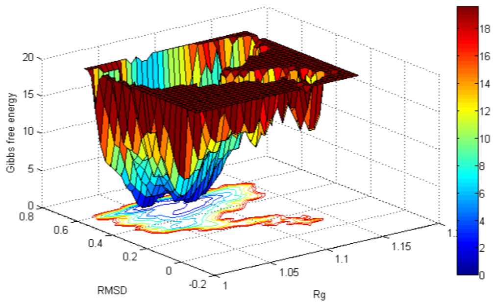
S. 7 3D Free Energy Landscape of the protein simulated system
