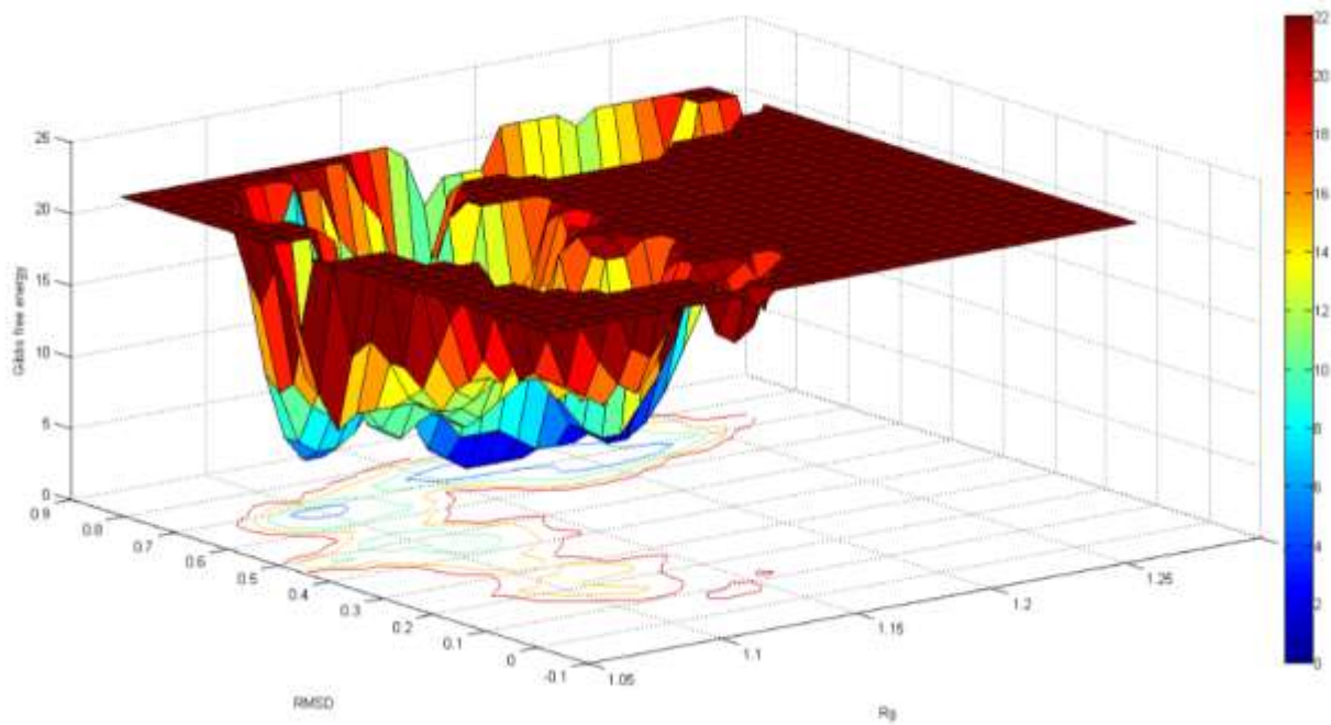
S. 8 3D Free Energy Landscape of the protein-SWCNT simulated system
