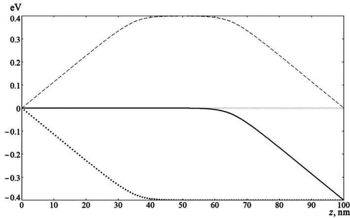
FIG. 3. Variation of electron potential energy profiles along the conductive channel of the transistor from source to drain: dashed curve – potential barrier \Delta E_0 in the absence of electric fields ( V_D = V_G = 0 ); dotted curve – the potential energy of electrons in the electric field u_\varphi at V_D = V_G = V_{G0} = 0.4 V; solid curve – total potential energy of electrons U at V_D = V_G = V_{G0} = 0.4 V
