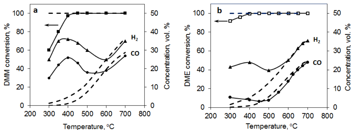
FIG. 2. Effect of temperature on DMM and DME conversions and H_2 and CO concentrations in DMM (a) and DME (b) partial oxidation over the Pt/CeO_2-ZrO_2 catalyst. Solid lines – experiment, dotted – thermodynamic equilibrium values
